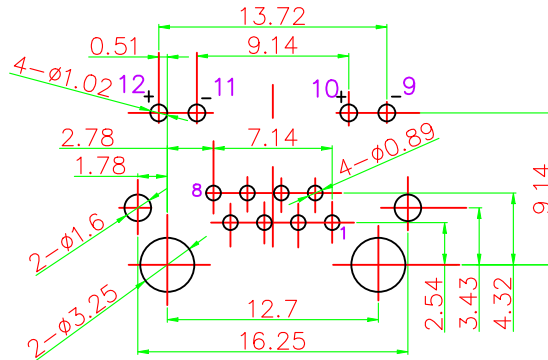
Recommended PCB layout (Component Side View)
